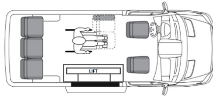
7 Passengers, 1 Wheelchair RWBS5
