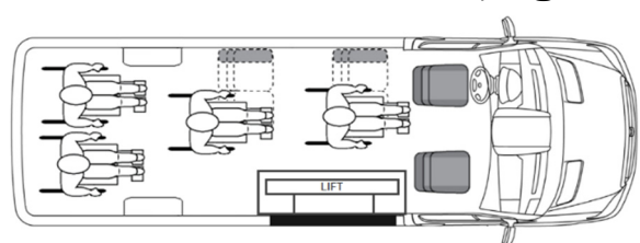
6 Passengers, 4 Wheelchairs ELCS1
