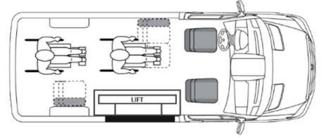
5 Passengers, 2 Wheelchairs RWBS3
