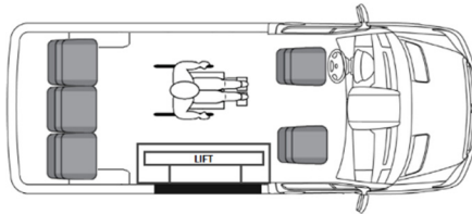
5 Passengers, 1 Wheelchairs RWBS2
