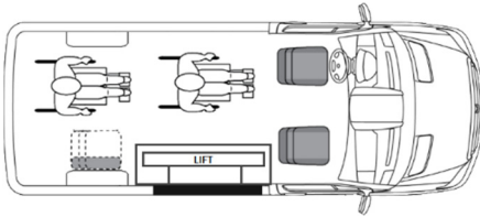
3 Passengers, 2 Wheelchairs RWBS1
