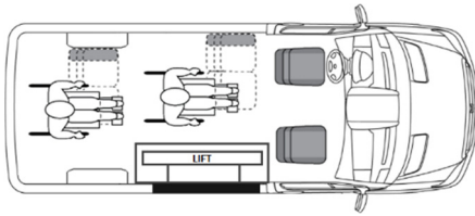
6 Passengers, 2 Wheelchairs RWBS4
