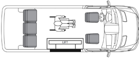
5 Passengers, 1 Wheelchair LWBS1
