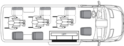
10 Passengers, 3 Wheelchairs ELS1
