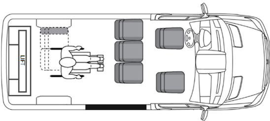
Rear Lift, 7 Passengers, 1 Wheelchairs RWBR3
