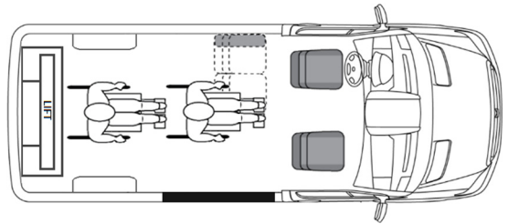
Rear Lift, 4 Passengers, 2 Wheelchairs RWBR4
