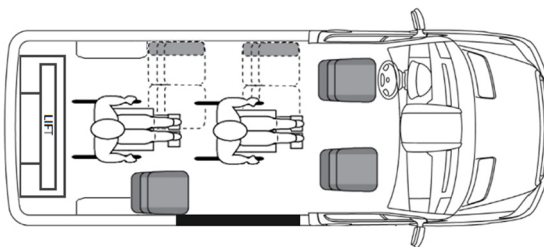
Rear Lift, 7 Passengers, 2 Wheelchairs RWBR7
