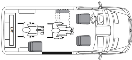
Rear Lift, 5 Passengers, 2 Wheelchairs RWBR5
